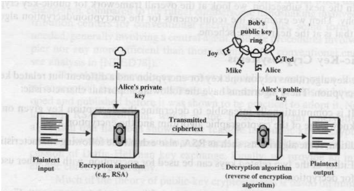
(a) Encryption
