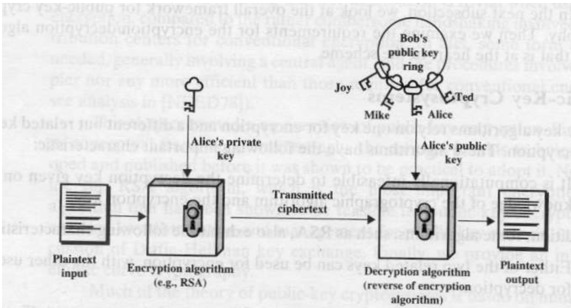
(b) Authentication
